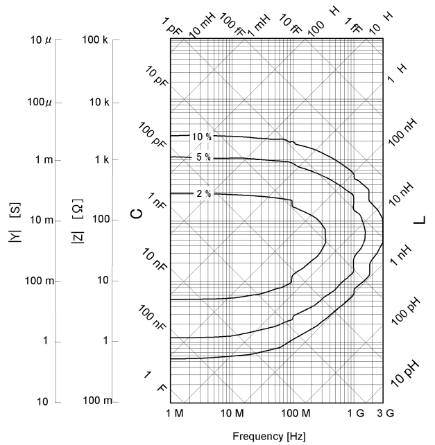
Figure 34. |Z| , |Y| Measurement accuracy when open/short/load calibration is performed. Oscillator level < -33 dBm. Point averaging factor \geq 8 within \pm 5 °C of calibration temperature.
