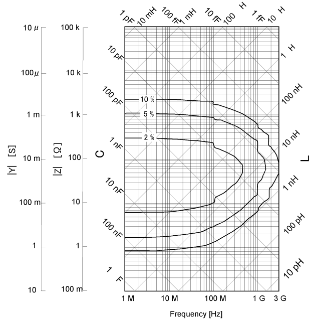
Figure 33. |Z| , |Y| Measurement accuracy when open/short/load calibration is performed. Oscillator level \geq -33 dBm. Point averaging factor \leq 7 within \pm 5 °C of calibration temperature.
