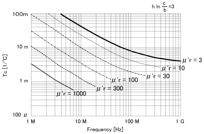
Figure 58. Typical frequency characteristics of temperature coefficient of \mu' (at F = 3 )
