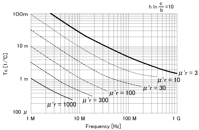
Figure 59. Typical frequency characteristics of temperature coefficient of \mu' (at F = 10 )
