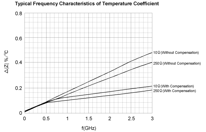
Figure 35. Typical frequency characteristics of temperature coefficient, (E_c + E_d)/\Delta T , when |Z_x| = 10 \Omega and 250 \Omega , E_{ah} = Z_{sh} = Y_{oh} = 0 are assumed 12 .
