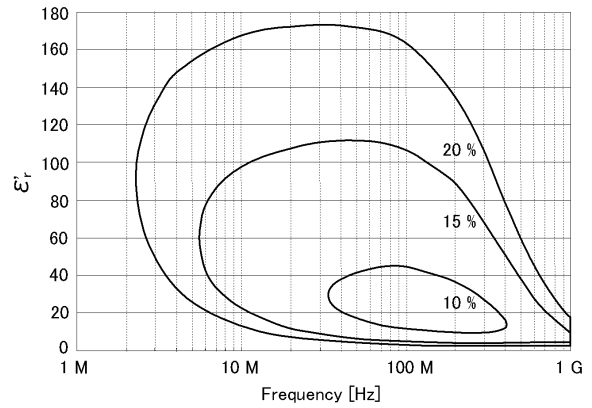
Figure 44. Permittivity ( \epsilon' ) vs. frequency (at t = 3 mm, typical)
