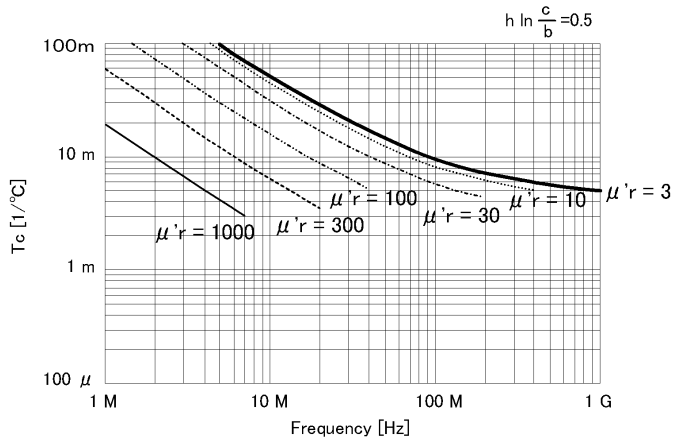
Figure 57. Typical frequency characteristics of temperature coefficient of \mu' (at F = 0.5 )
