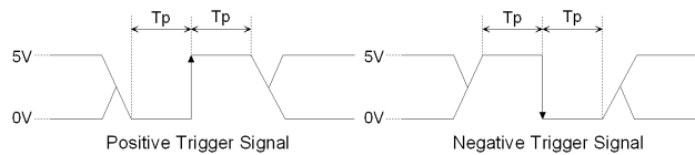
Figure 6. Definition of pulse width ( T_p )
