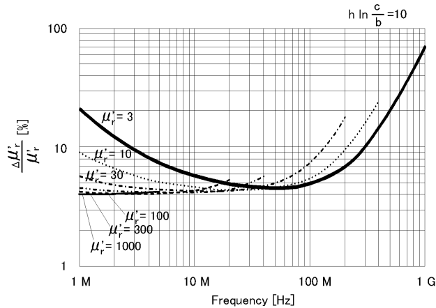
Figure 47. Permeability accuracy \frac{\Delta\mu'_r}{\mu'_r} vs. frequency (at F = 10 , typical)
